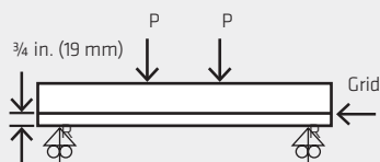
Schematic Diagram of the Beam Fatigue Test
