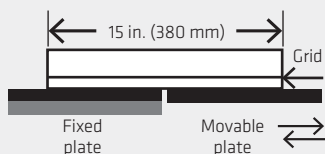
Schematic Diagram of the Overlay Test
