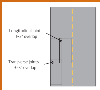
FIGURE 17: Overlapping GlasGrid across transverse or longitudinal joint
