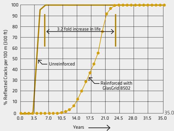
FIGURE 10: Estimated life of GlasGrid reinforced vs. unreinforced overlay for a typical composite pavement structure.
