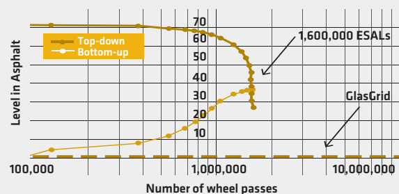
FIGURE 12: Reinforced crack development plot.
