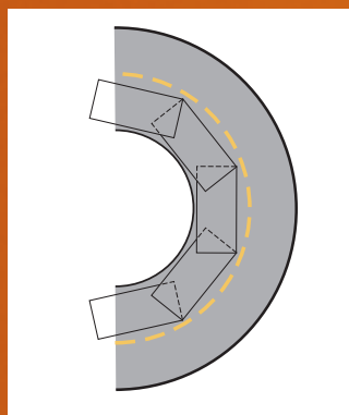
FIGURE 16: Cutting and overlapping GlasGrid around a curve
